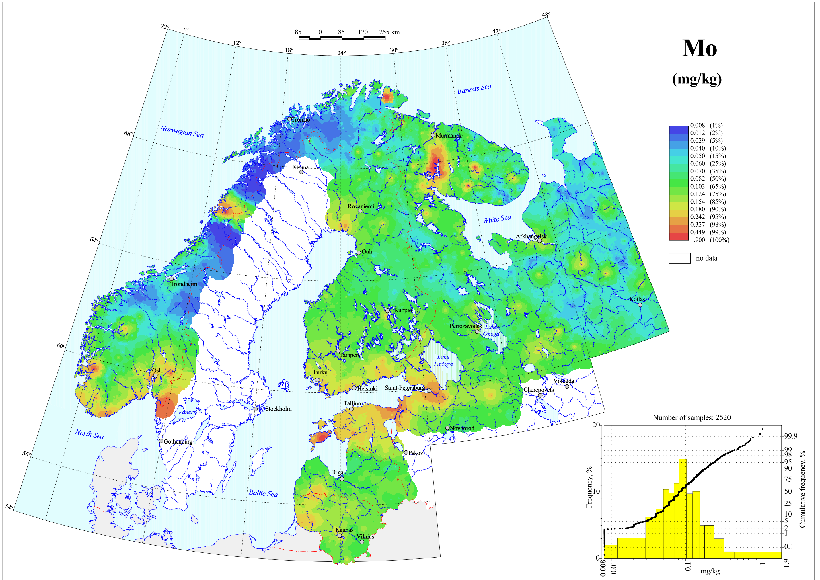
Molybdenum in Terrestrial Moss, Total Content
